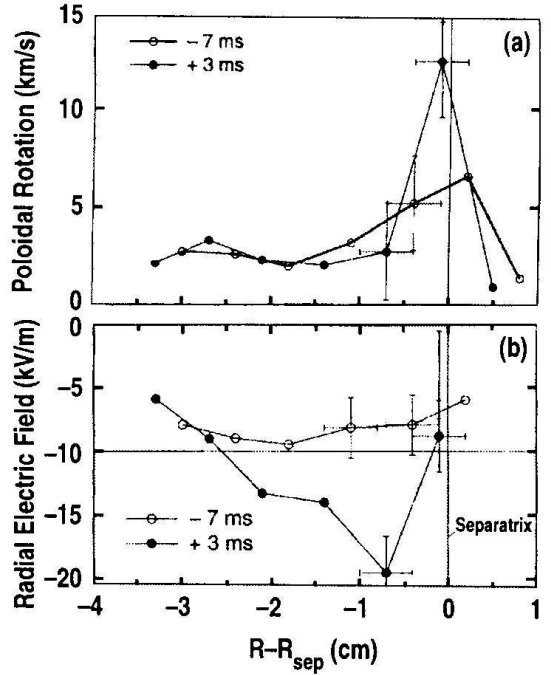
Figure 4: The main ion poloidal rotation (a) and radial electric field profile (b) computed using measured quantities for 7 ms before and 3 ms after L-H transition in DIII-D. 18
