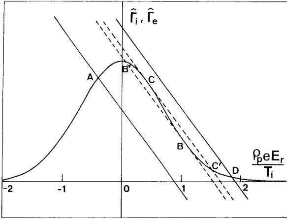
Figure 3: Normalized ion and electron fluxes vs the radial electric field. Dashed lines indicate the bifurcation condition. 15
