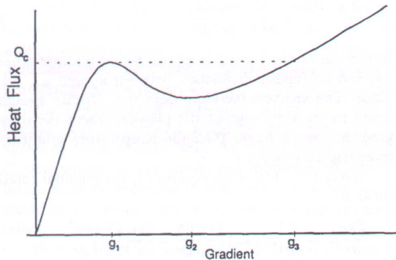
Figure 6: Local heat flux versus temperature gradient. 20
