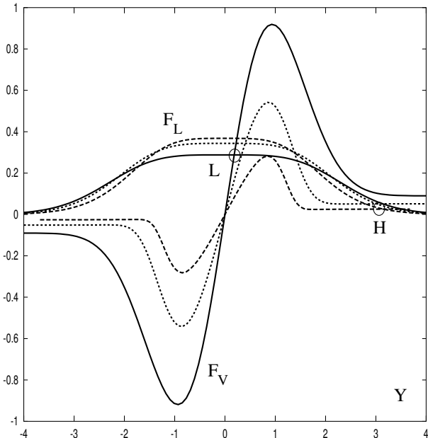
Figure 5: Normalized forces applied to the ions in the poloidal direction vs the parameter Y related to radial electric field. Ion temperature increases from solid through dotted to dashed curves. 17
